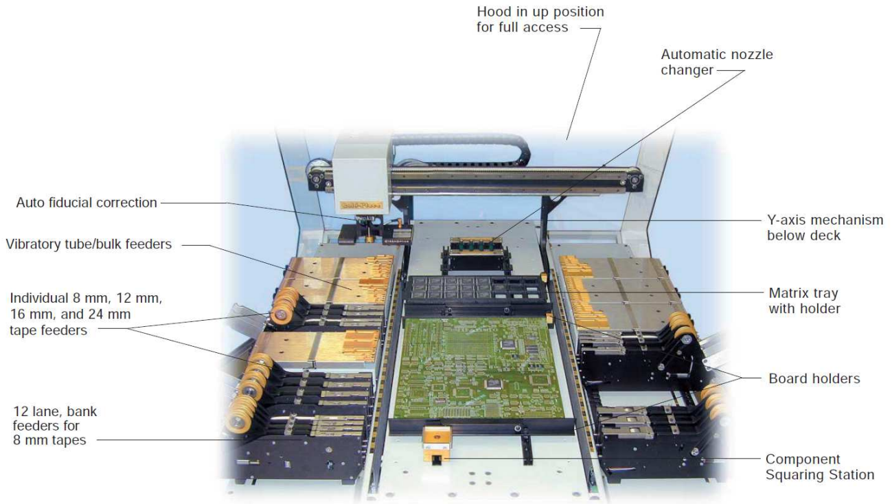
Model L60 showing easily accessible, unobstructed work deck
